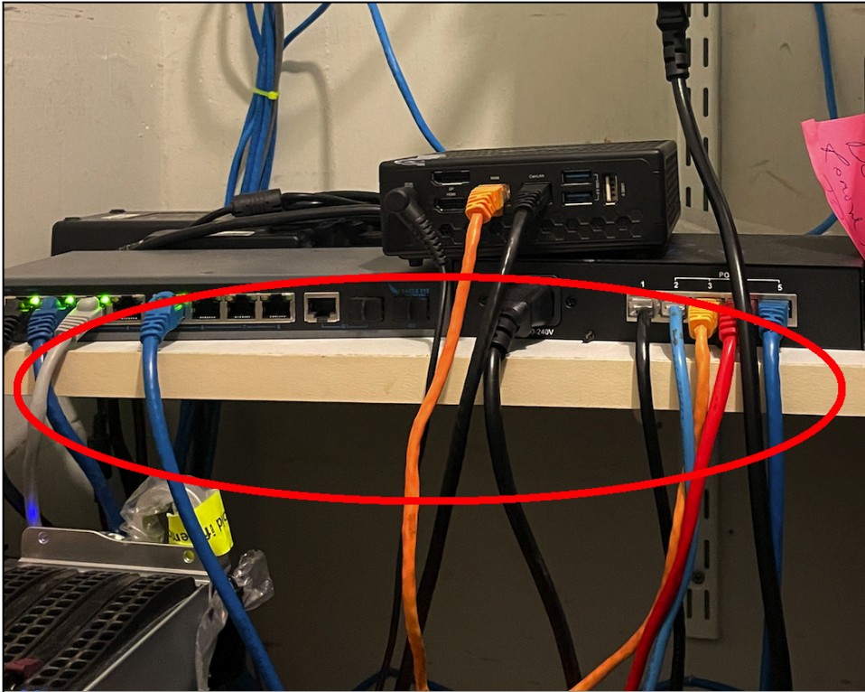
BAD EXAMPLE: DO NOT leave cables hanging loose. Always secure them to each other and the wall.
