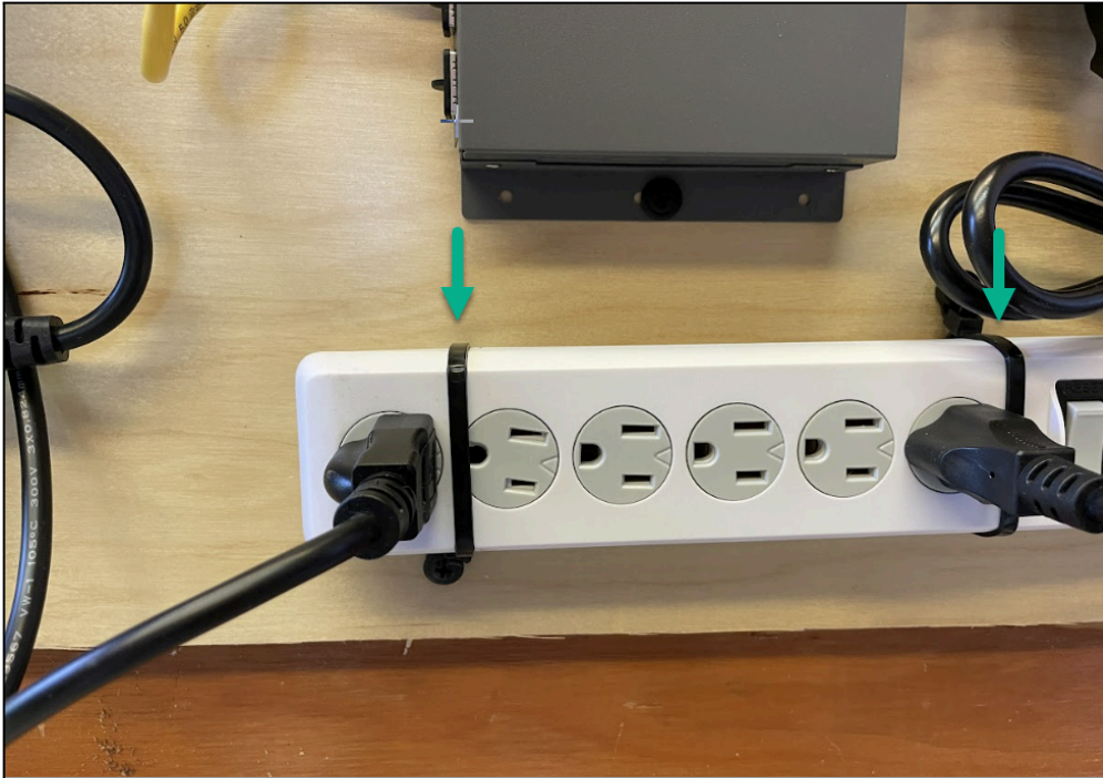
GOOD EXAMPLE: Do securely mount the power strip.
