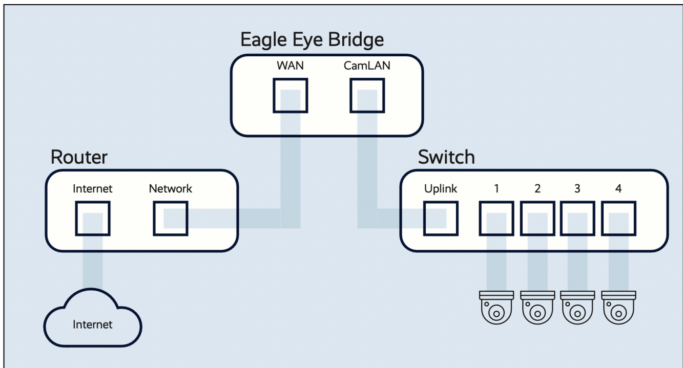
Typical wiring diagram for an Eagle Eye Bridge/CMVR
