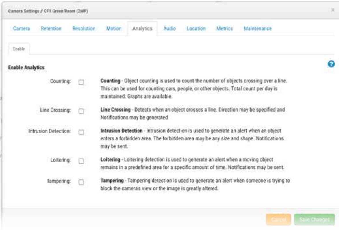
Image 2: Analytics tab within camera settings
