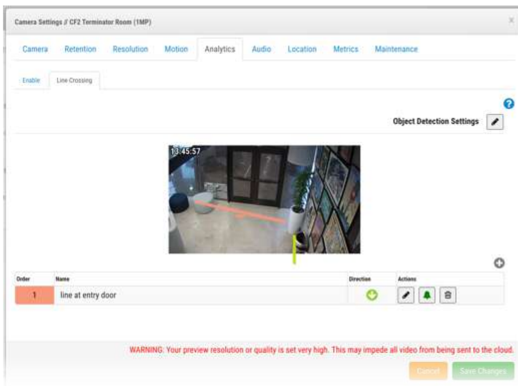
Image 6: Example setup of the Line Crossing Analytic with the line in the center of the camera view.
